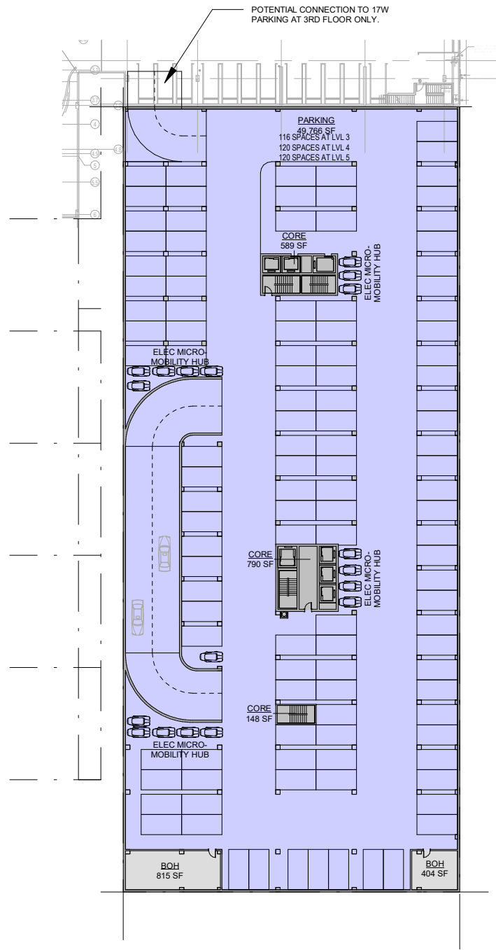
3RD, 4TH AND 5TH FLOOR PLAN (3 FULL PARKING LEVELS)
