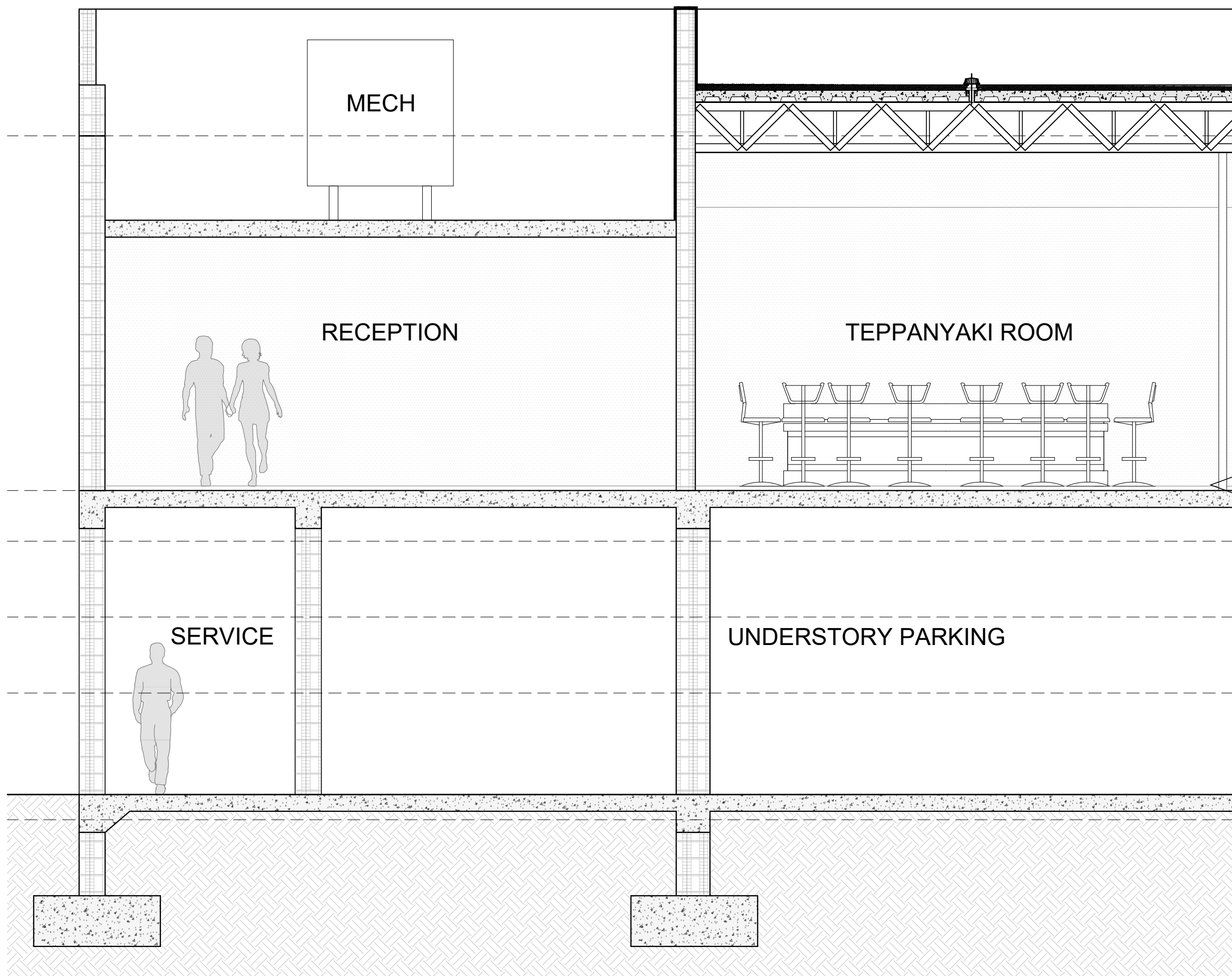
1 ENGLARED SECTION: MECHANICAL WELL SCALE: 1/4" = 1'-0"
