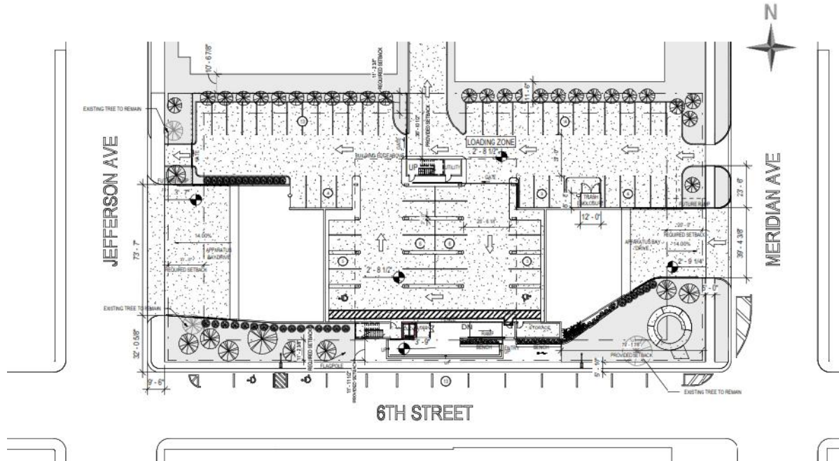
Figure 2: Site Plan
