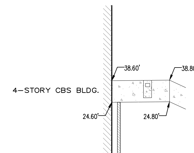
DETAIL "A" FRONT VIEW Scale: 1"=20'
