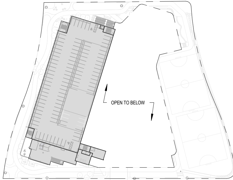
LEVEL 02 FAR = 40,760 sf.
