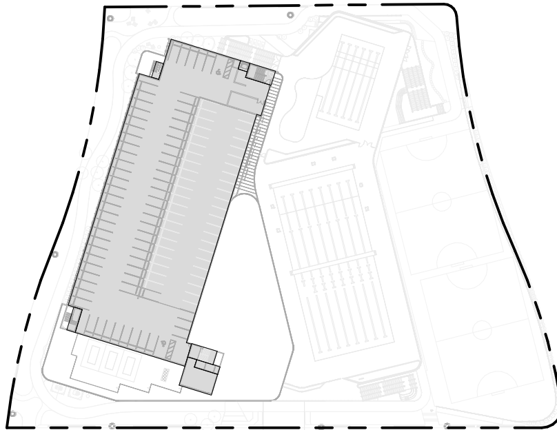
LEVEL 05 FAR = 35,810 sf.
