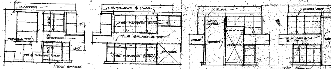
KITCHEN ELEVATIONS SCALE 3/8" = 1'-0"
