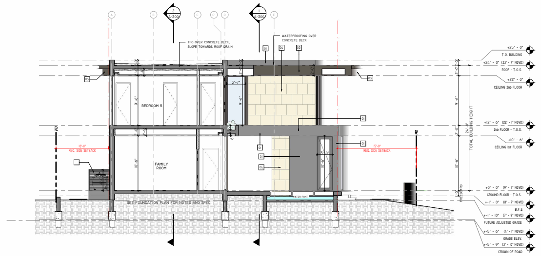
GRAPHIC SCALE 3/16" = 1'-0" 1 SECTION C
