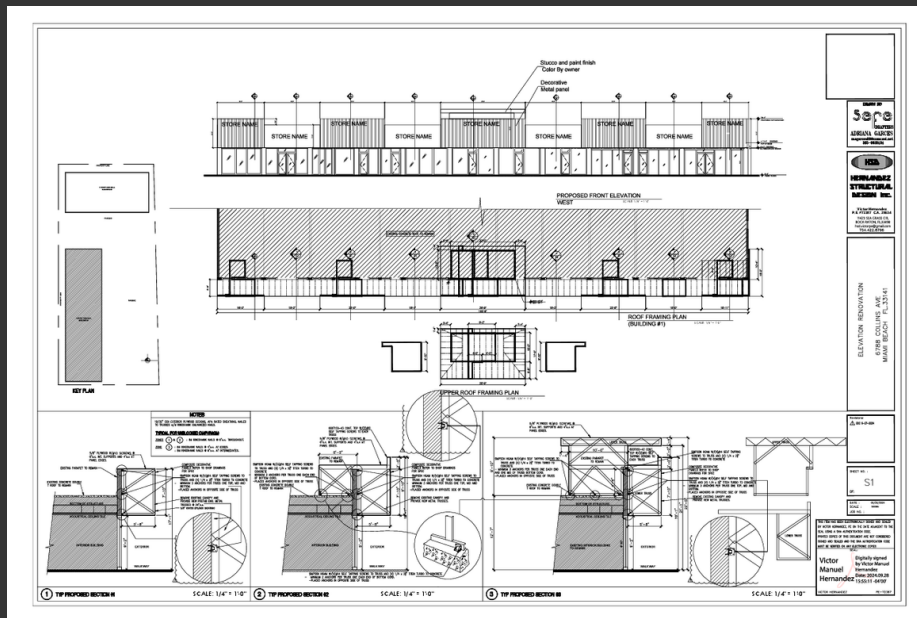
Images: Elevation Renovation A1.1, A -1, S1, S2, Front Elevation Renovation
