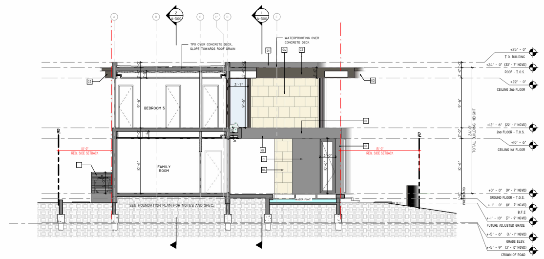
GRAPHIC SCALE 3/16" = 1'-0" SECTION C
