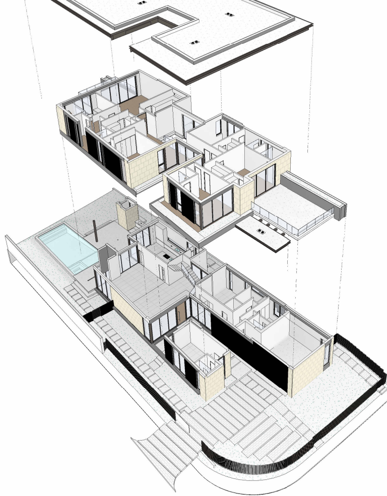
1 EXPLODED AXONOMETRIC DIAGRAM 1
