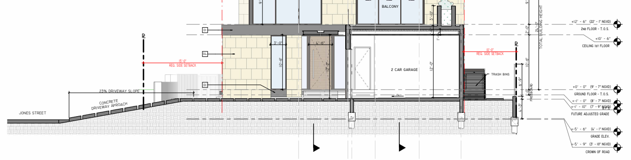
GRAPHIC SCALE 0 5 10 20 3/16" = 1'-0" 1/2" = 1'-0" SECTION E
