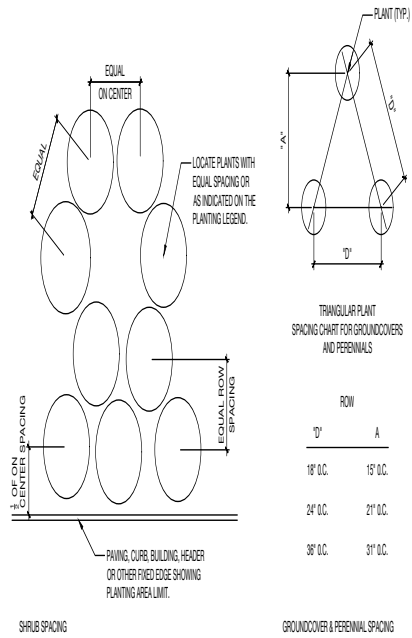
6 PLANT & SHRUB SPACING DETAIL SCALE: 3/32" = 1'-0"
