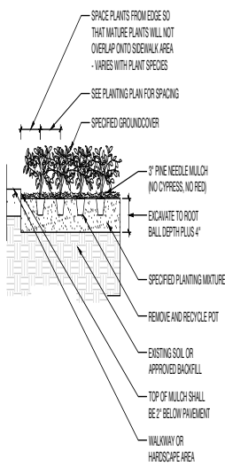
5 GROUND COVER PLANTING DETAIL SCALE: 3/32" = 1'-0"
