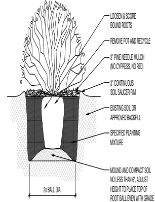
3 SHRUB PLANTING DETAIL SCALE: 3/32" = 1'-0"
