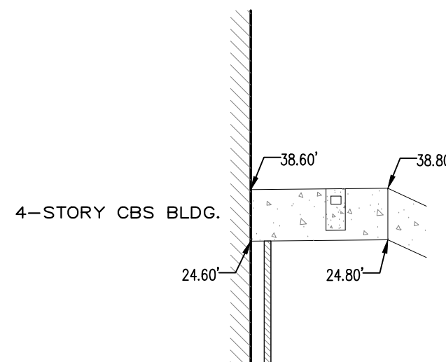
DETAIL "A" FRONT VIEW Scale: 1"=20'
