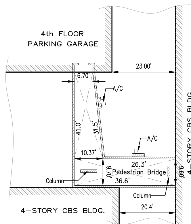
DETAIL "A" TOP VIEW Scale: 1"=20'
