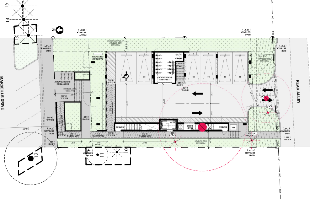
EXISTING TREE DISPOSITION PLAN (1.01) SCALE: 1" = 20'-0"
