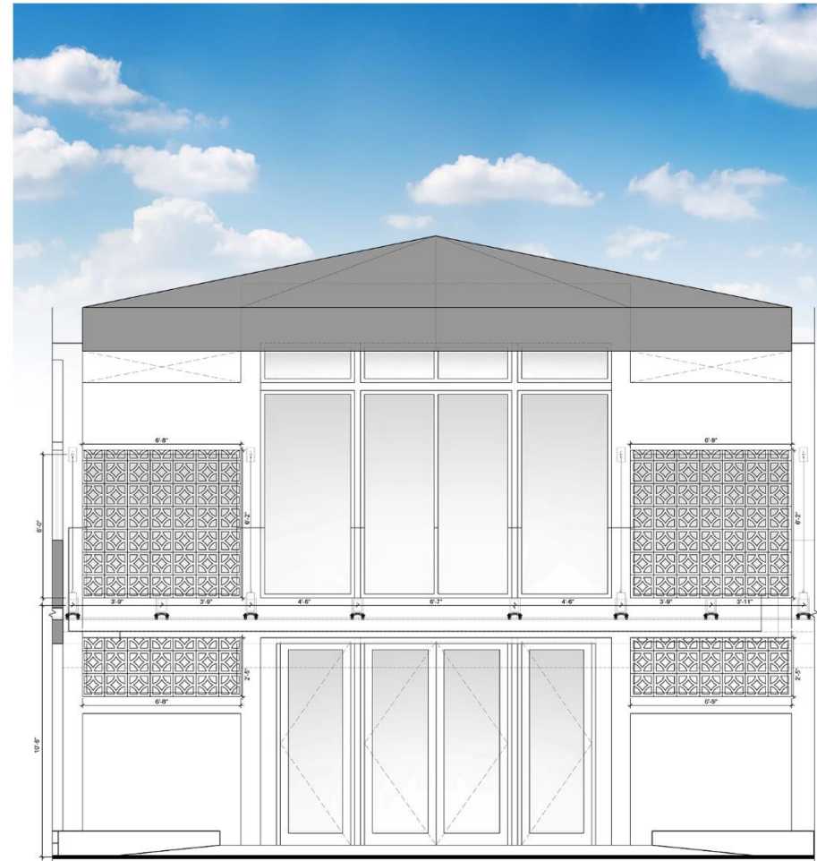
A4 ENLARGED EAST ELEVATION
