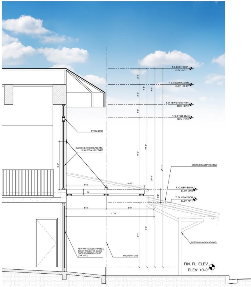
A1 PROPOSED 1 - FRONT ENTRY SECTION (19'-5" CANOPY)
