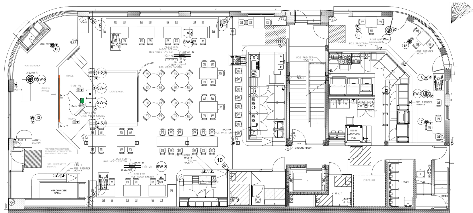
E VIDEO & SOUND AND POS / PRINTERS ( WALL AND CEILING MOUNTED) GROUND FLOOR PLAN SCALE: 1/4" = 1'-0"
