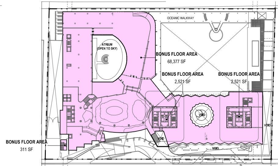
1 FAR DIAGRAM - LV02 LOBBY 1" = 80'-0"
