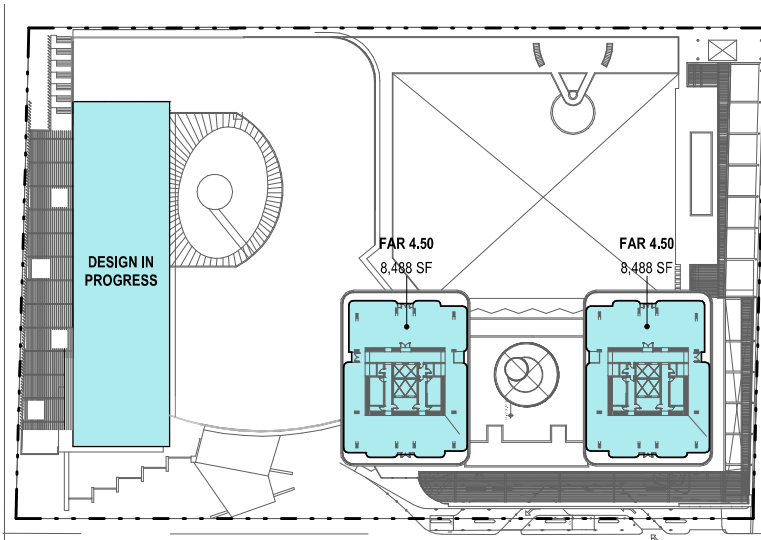
2 FAR DIAGRAM - LV 08 RESIDENTIAL 1" = 80'-0"
