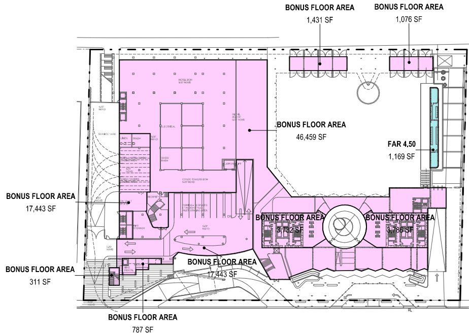
2 FAR DIAGRAM - LEVEL 01 1" = 80'-0"
