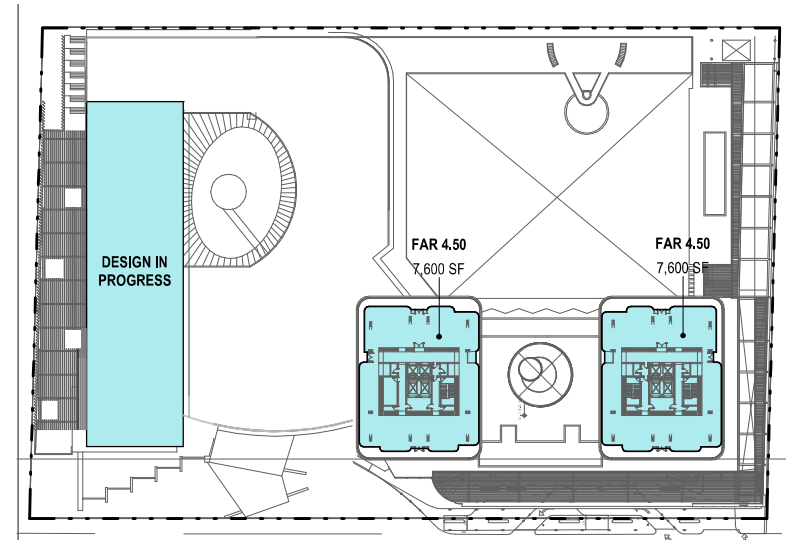
1 FAR DIAGRAM - LV 07 RESIDENTIAL 1" = 80'-0"
