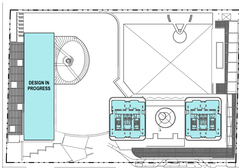
2 FAR DIAGRAM - LV05 SPA HOTEL 1" = 80'-0"
