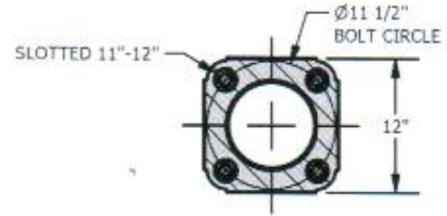
SECTION B-B SCALE 0.06 : 1
