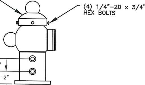
SECTION (SCALE 2:1)
