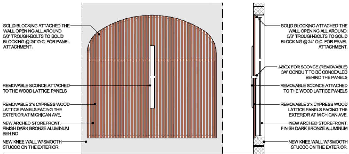
Details of the proposed wood panel system, Sheet A301
