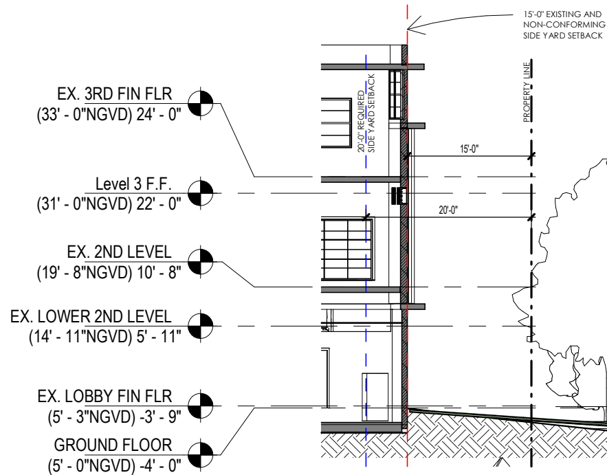
2 REQUIRED FRONT YARD SECTION 1/16" = 1'-0"
