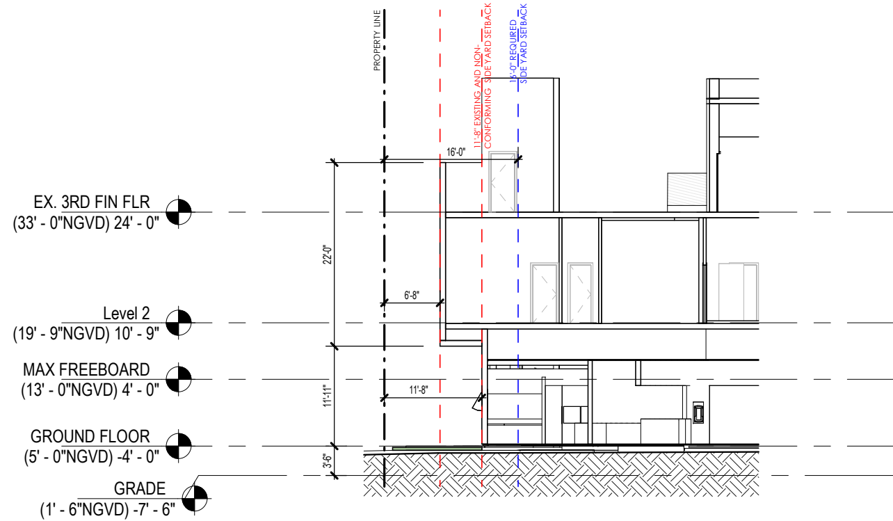
1 REQUIRED SIDE YARD SECTION 1/16" = 1'-0"
