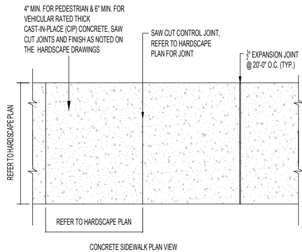
CONCRETE SIDEWALK PLAN VIEW
