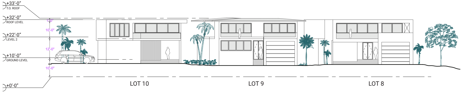
STREET VIEW ELEVATION
