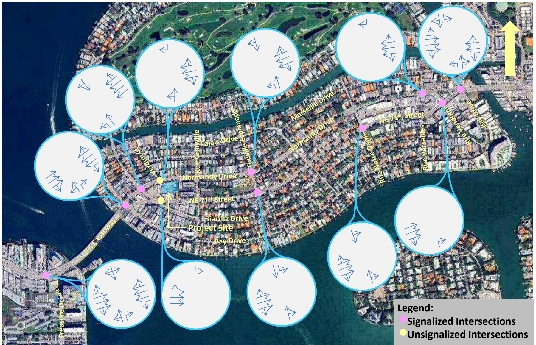
Figure 3 – Intersection Geometry/Permitted Movements 1960 Normandy Drive City of Miami Beach, Florida
