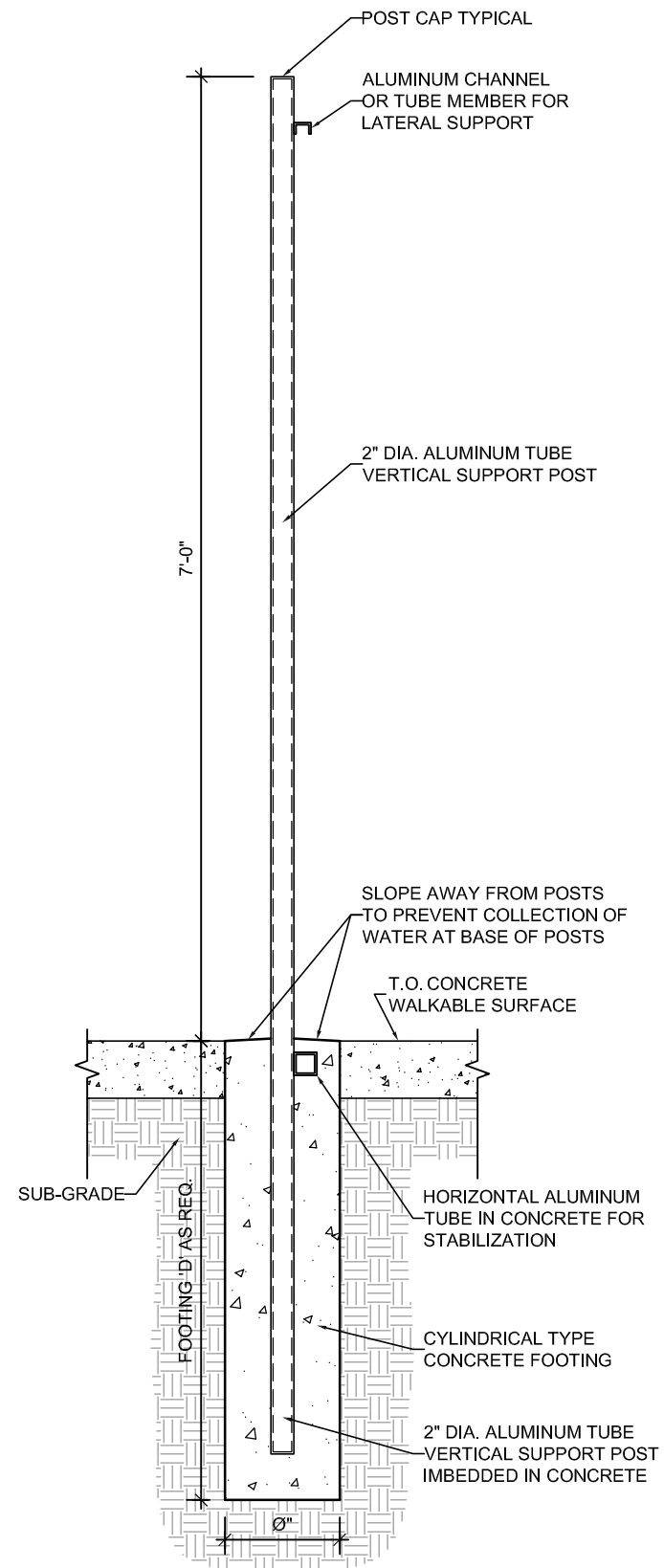
FENCE SECTION THRU VERTICAL SUPPORT POSTS
