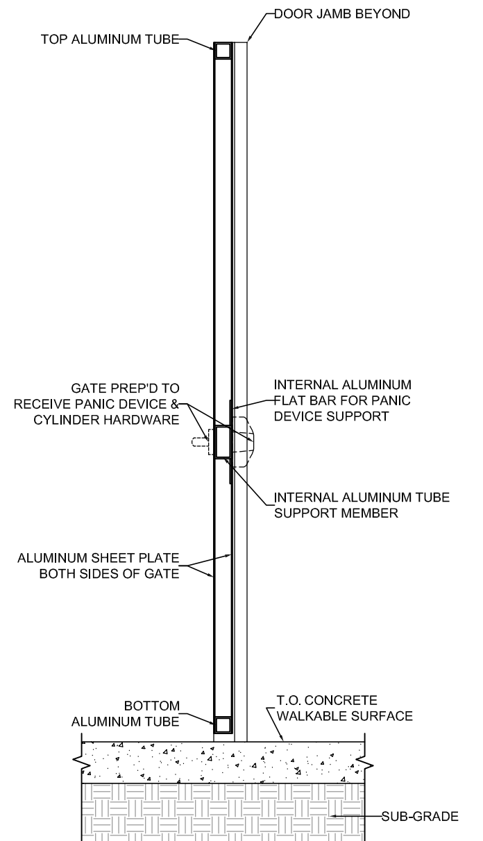
GATE SECTION
