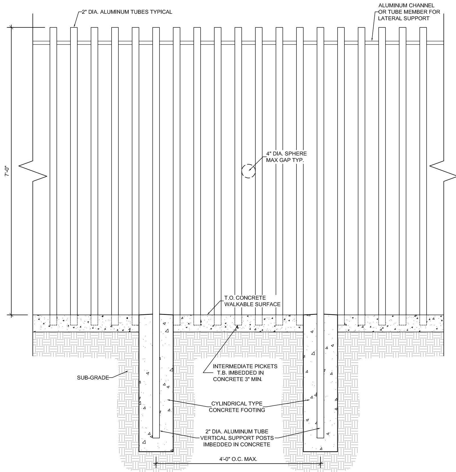
FENCE ELEVATION/SECTION
