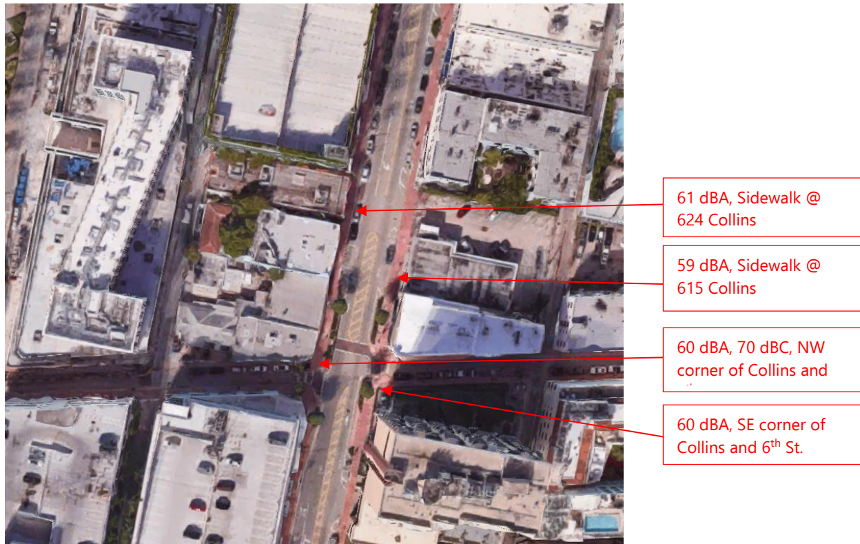
Figure 4 - Map of Ambient Noise Measurement Results
