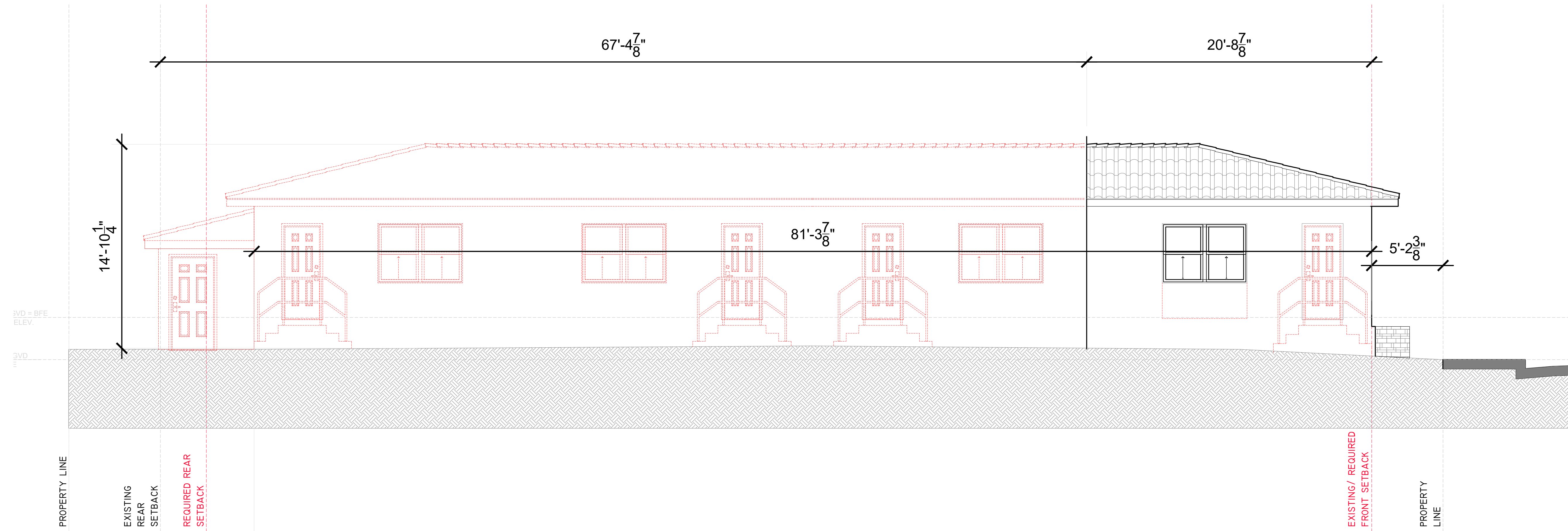
1. WEST ELEVATION
