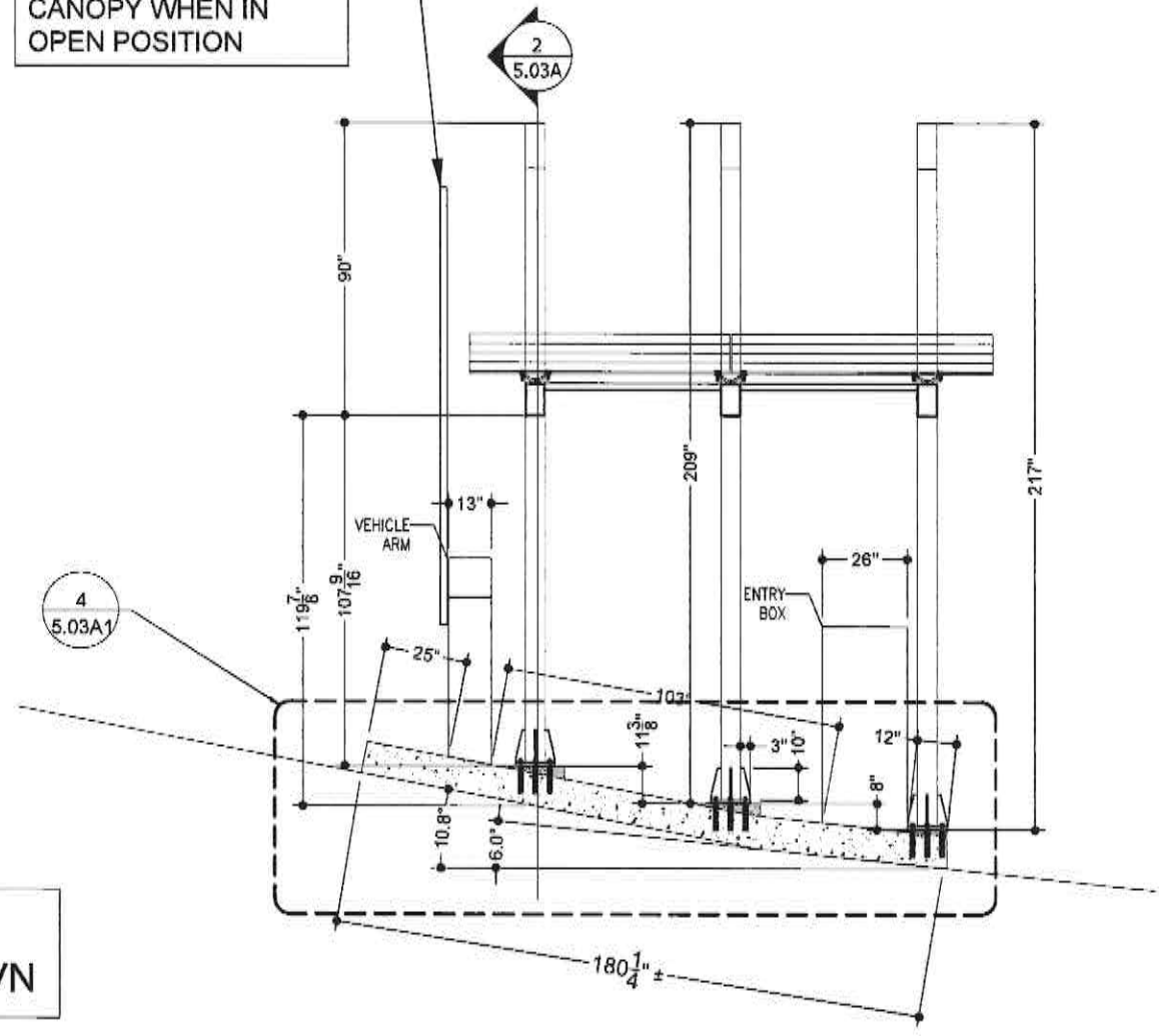
3 CANOPY 3 ELEVATION
