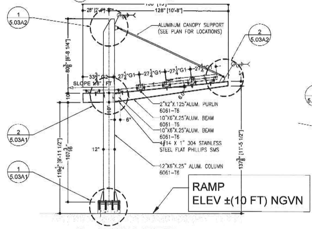
2 CANOPY 3 SECTION
