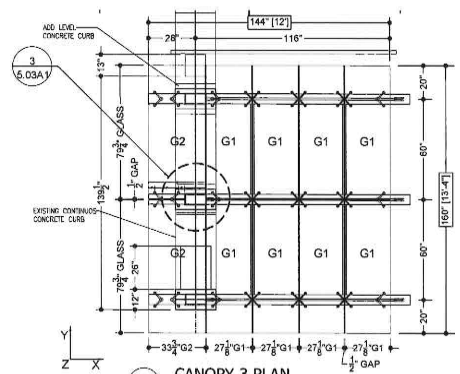
1 CANOPY 3 PLAN
