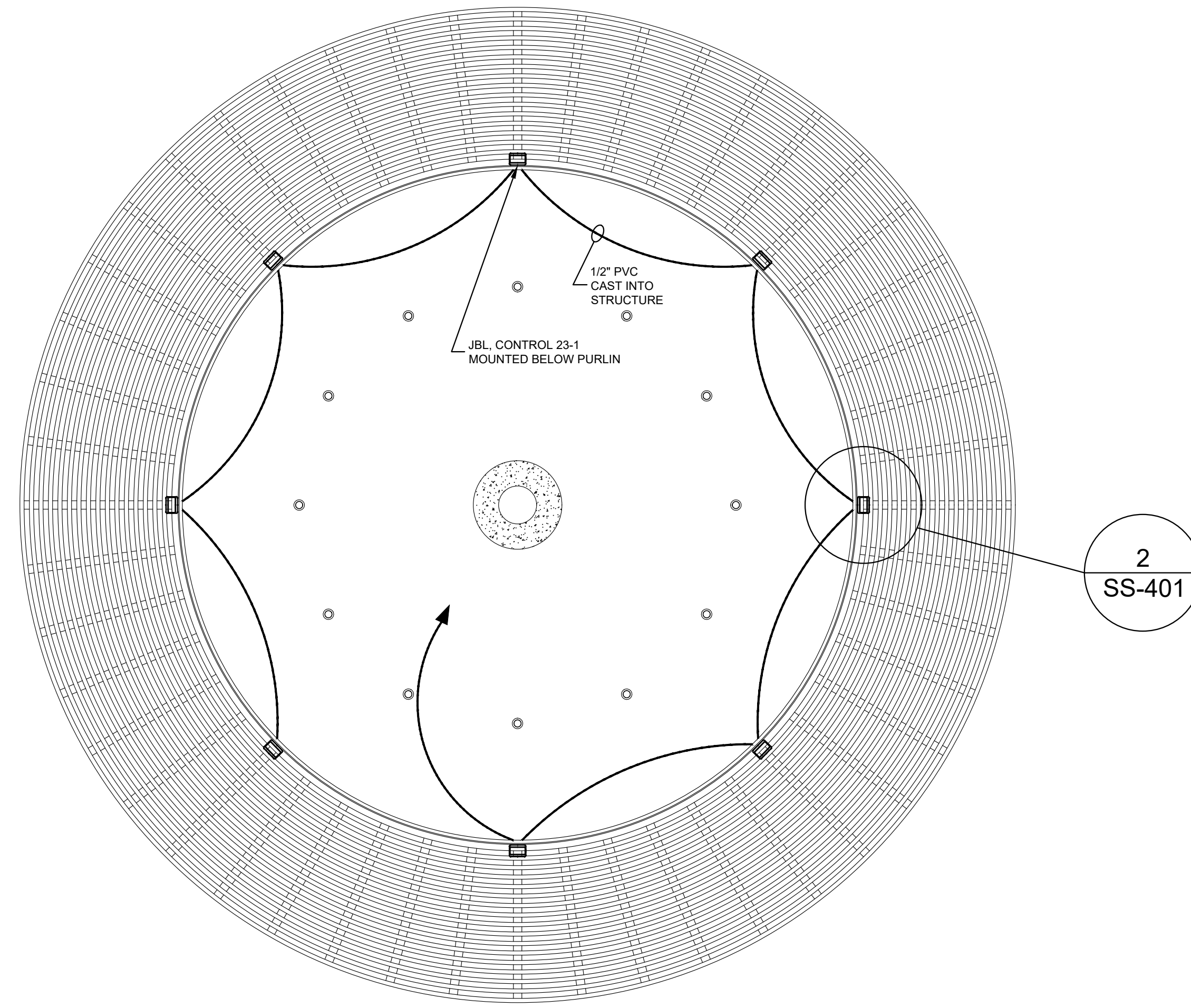
1 SS-401 POOL BAR CEILING STRUCTURE PLAN - SPEAKER MOUNTING LOCATIONS AND CONDUIT LAYOUT SCALE: 1/4"=1'-0"
