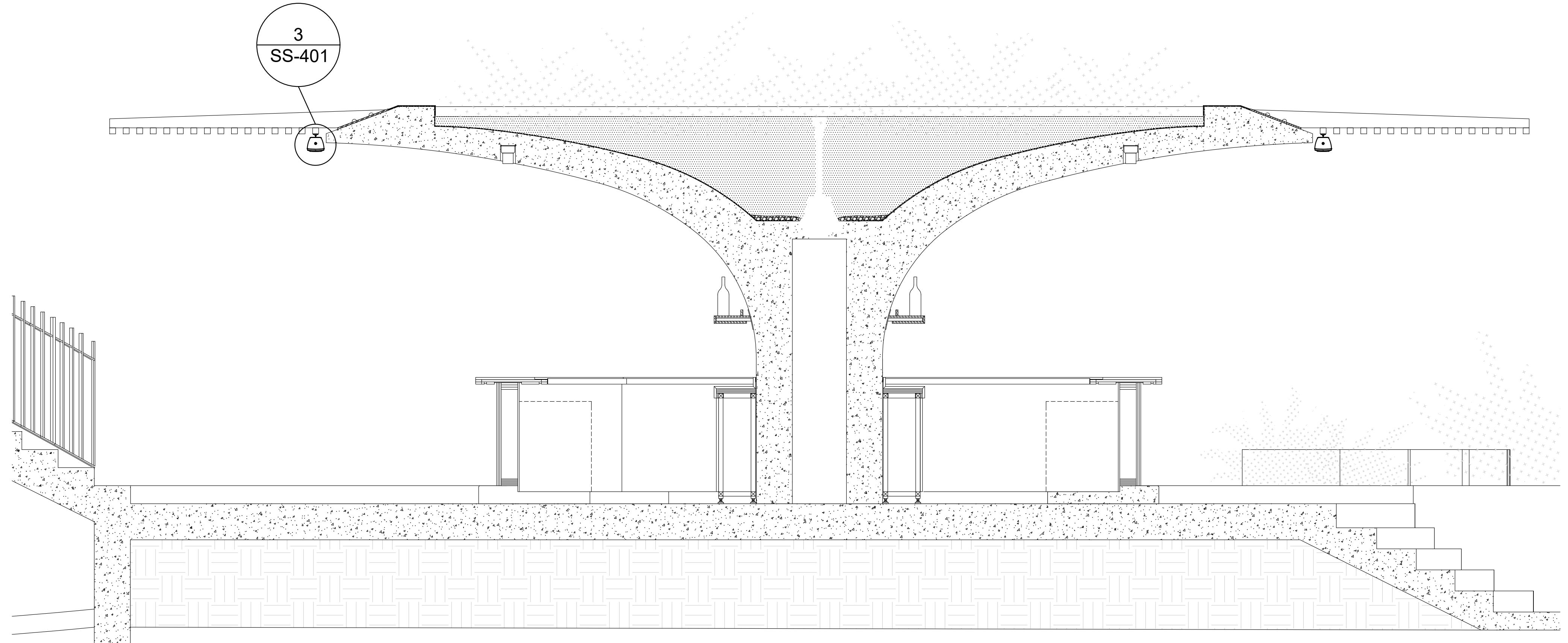
2 SS-401 POOL BAR CEILING STRUCTURE ELEVATION - SPEAKER MOUNTING LOCATIONS SCALE: 1/2"=1'-0"
