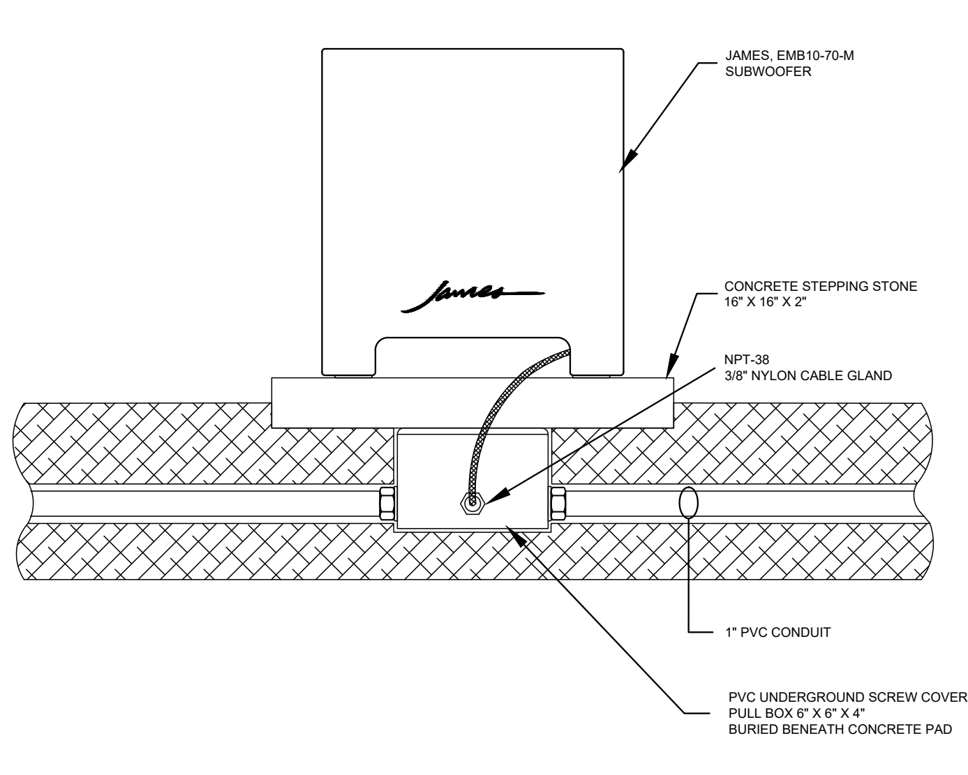
1 SS-402 LANDSCAPE SUBWOOFER MOUNTING DETAIL - JAMES EMB10-70-M SCALE: 3/16"=1'-0"
