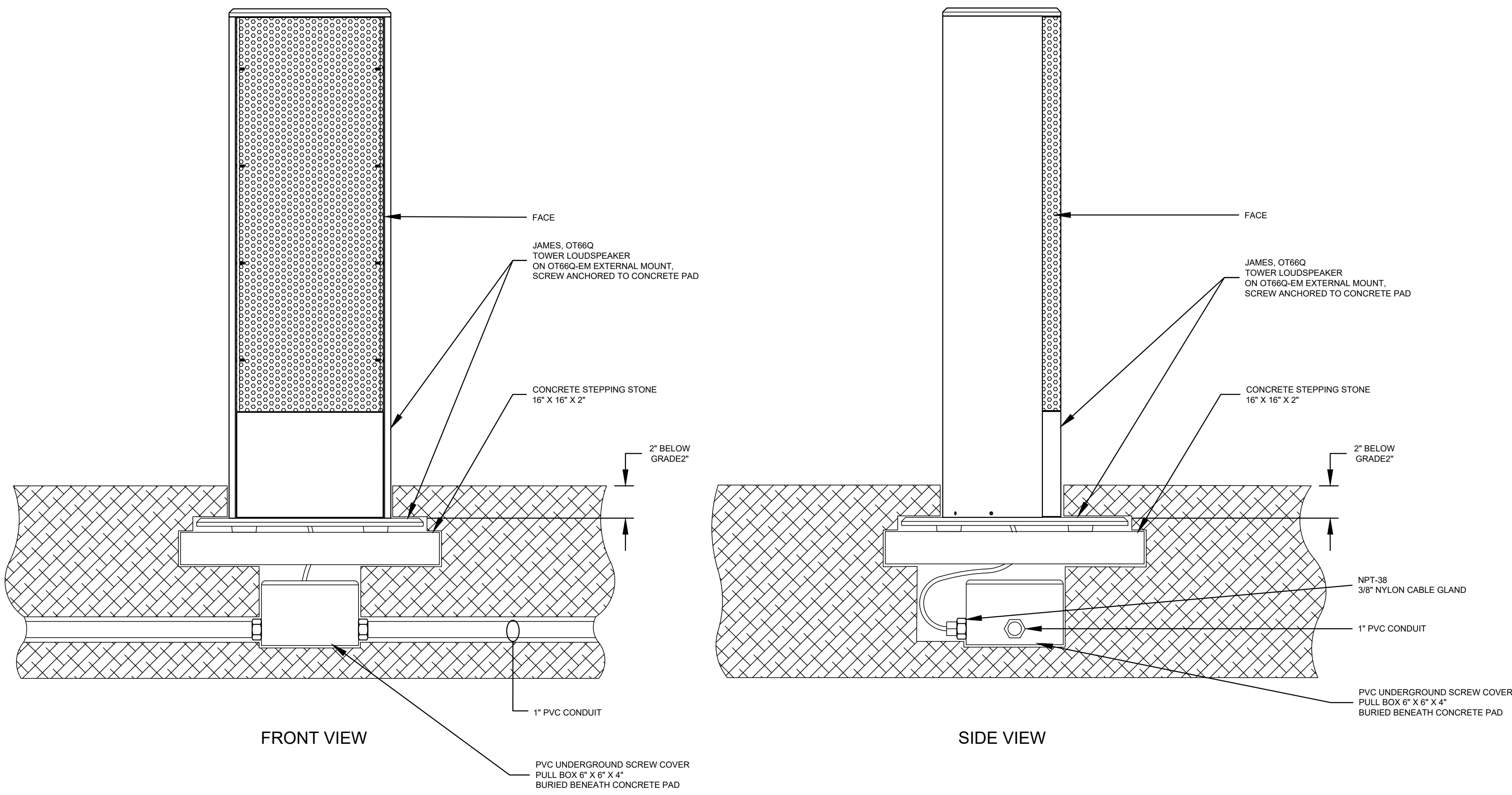
3 SS-402 LANDSCAPE TOWER MOUNTING DETAIL - JAMES OT86Q SCALE: 3/16"=1'-0"
