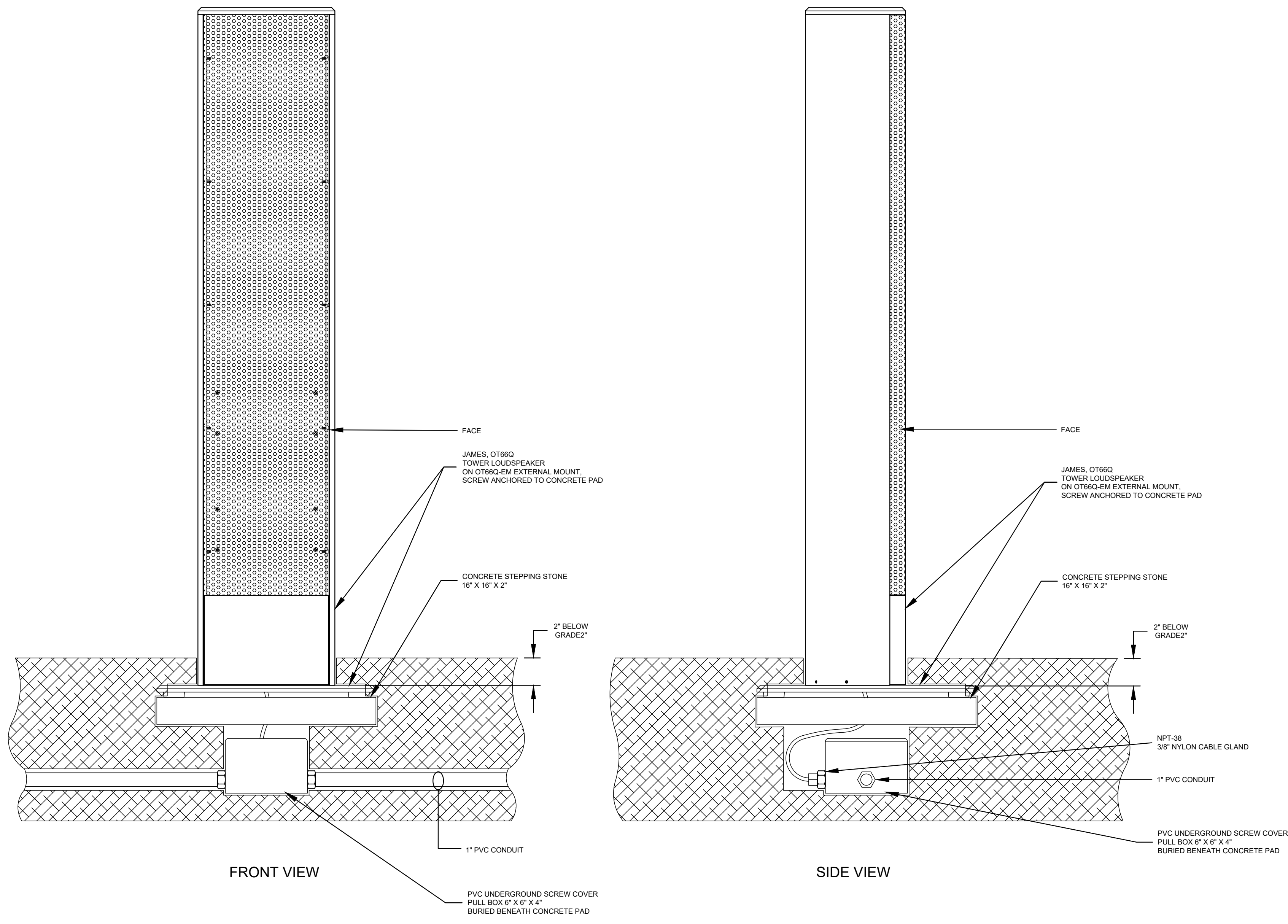
4 SS-403 LANDSCAPE TOWER MOUNTING DETAIL - OT88Q SCALE: 3/16"=1'-0"
