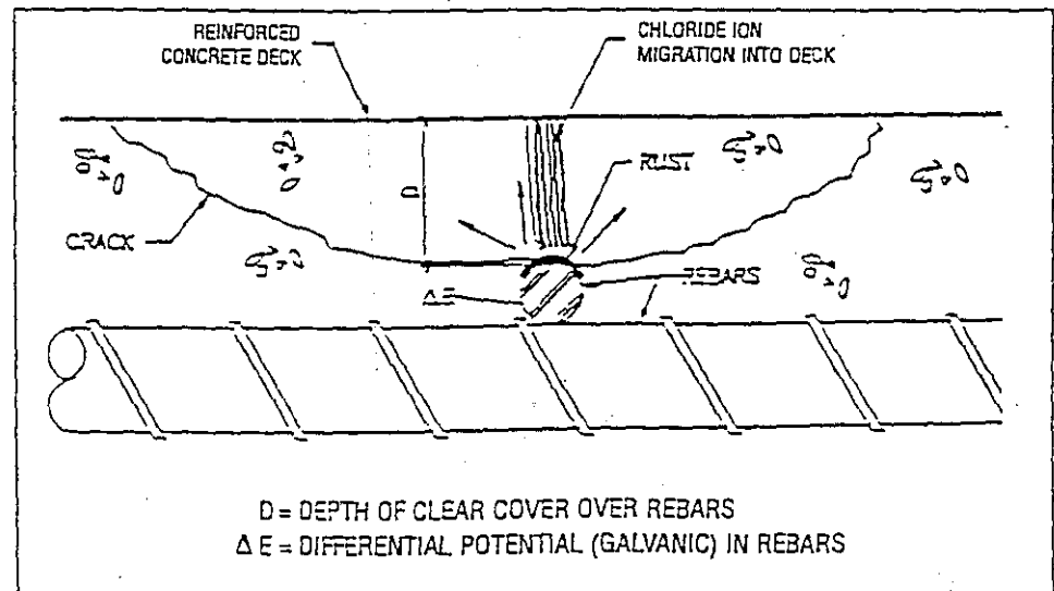
Figure 1 - Rebar corrosion spalling mechanism
