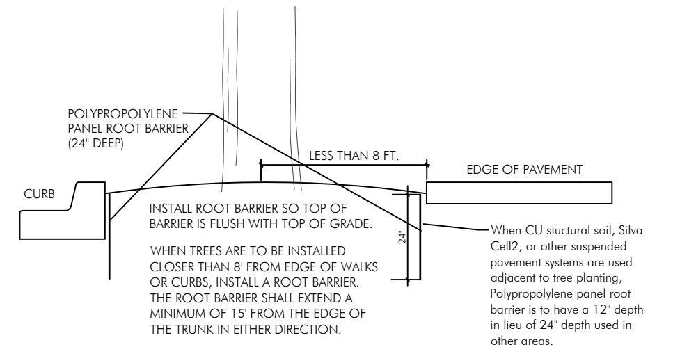
ROOT BARRIER INSTALLATION DETAIL
