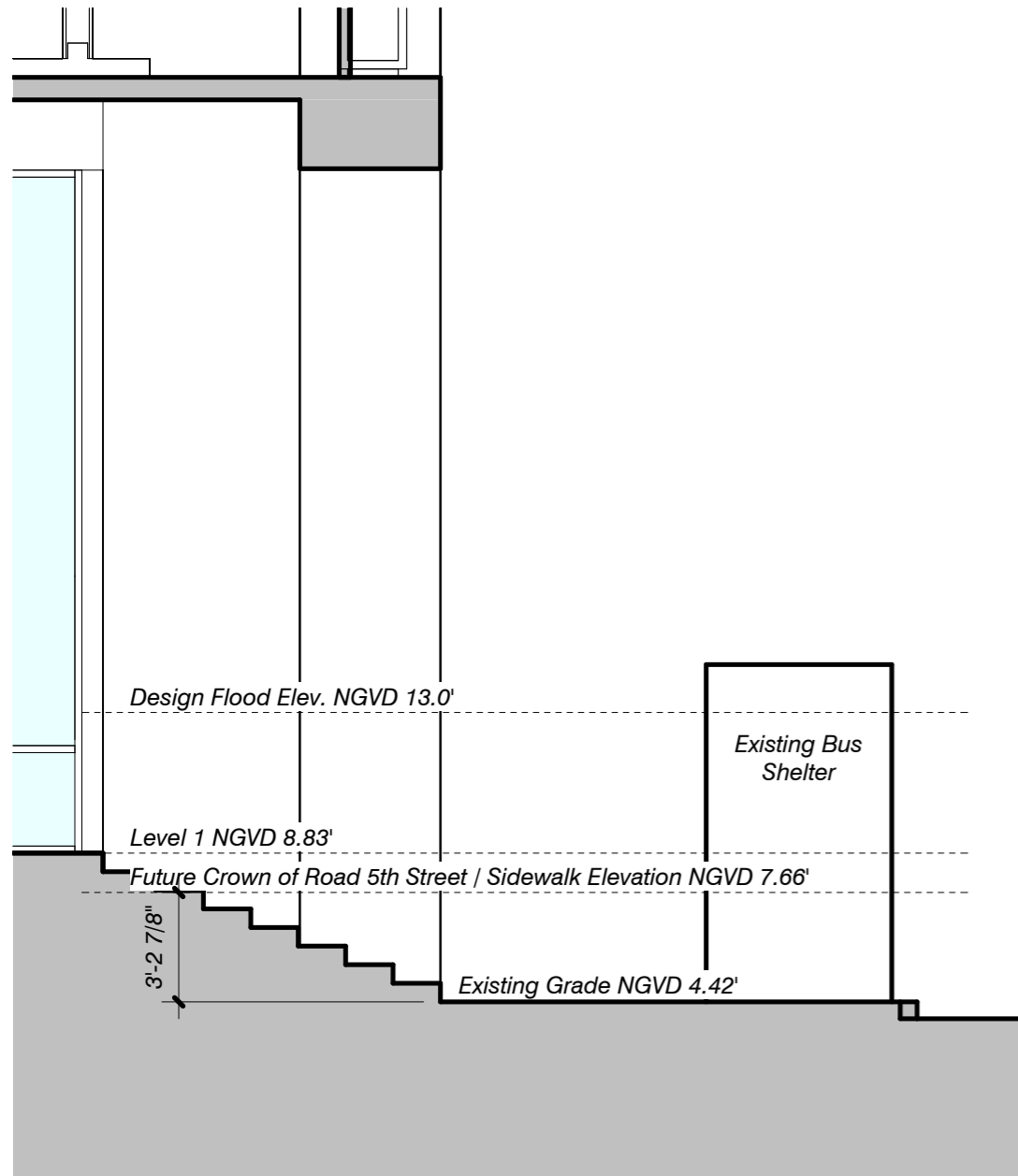
Section Through Sidewalk
