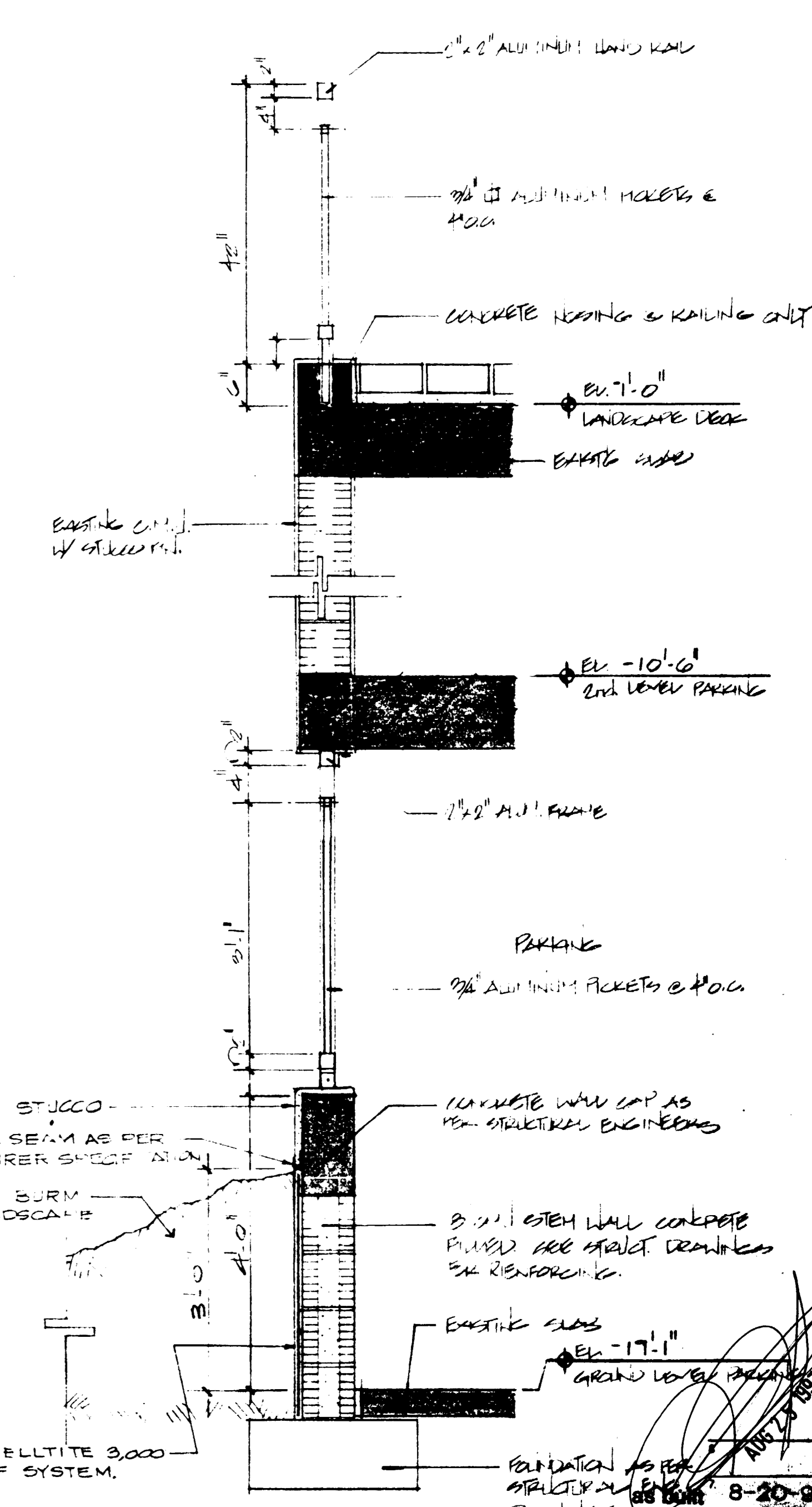
1 wall section 3/4"
