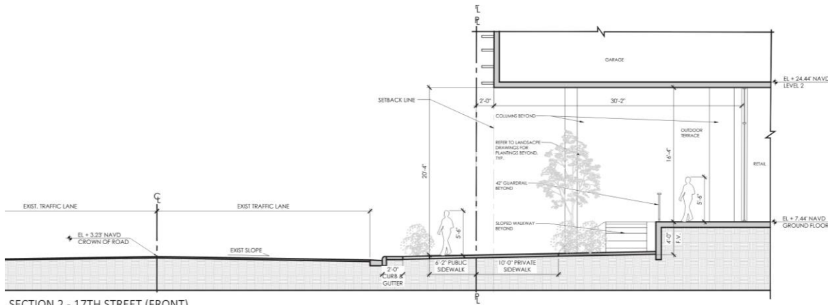
SECTION 2 - 17TH STREET (FRONT)
