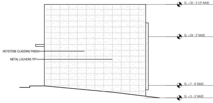
TRANSFORMER VAULT WEST ELEVATION
