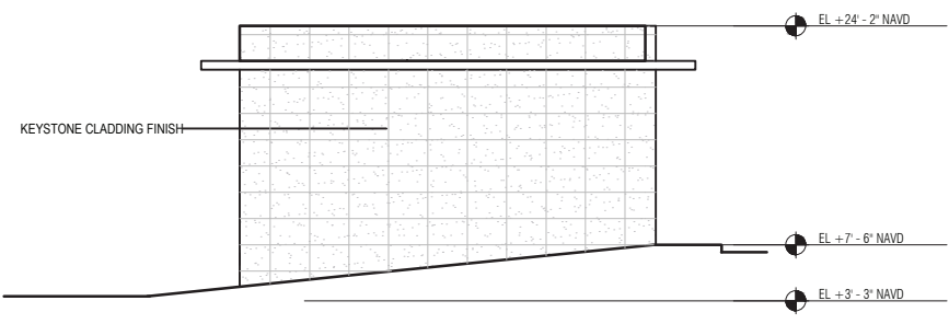
TRANSFORMER VAULT EAST ELEVATION
