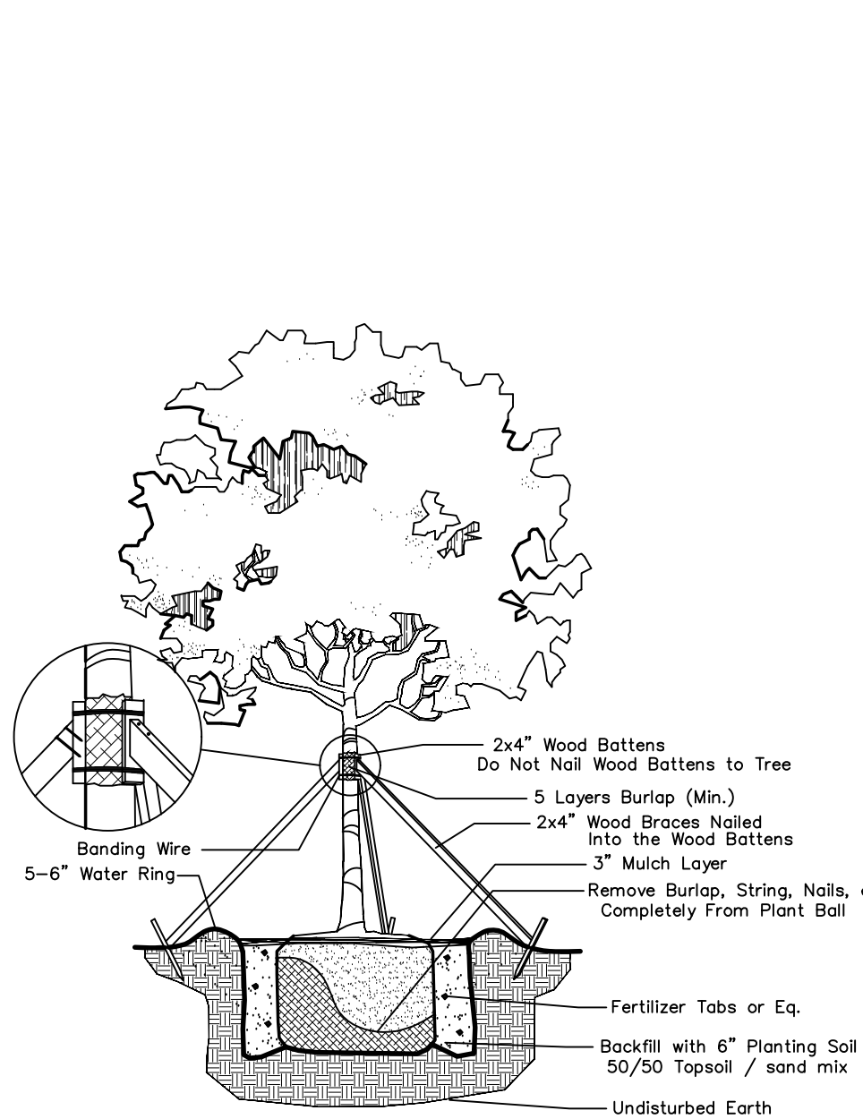
Large Tree Planting Detail
