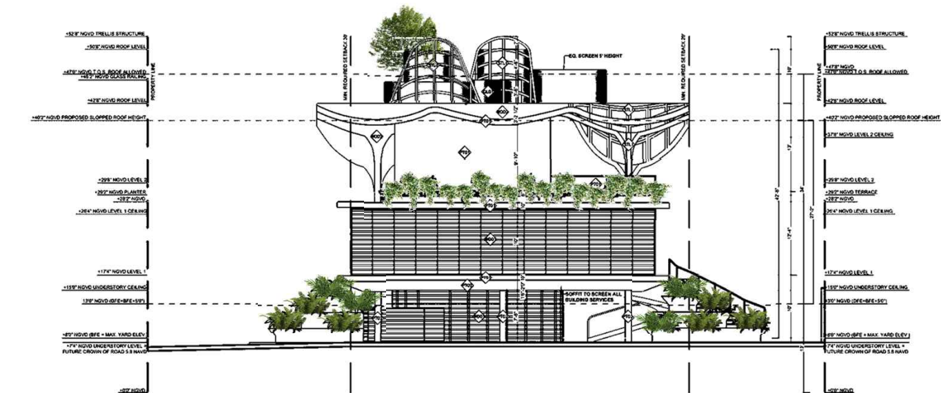
2 A301 NORTHEAST EXTERIOR ELEVATION 1/16" = 1'-0"
