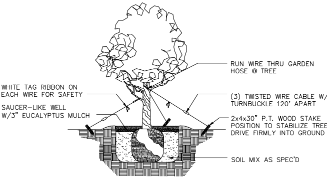
SMALL TREE SUPPORT DETAIL
