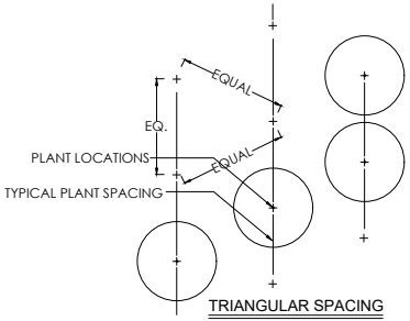
TRIANGULAR SPACING
