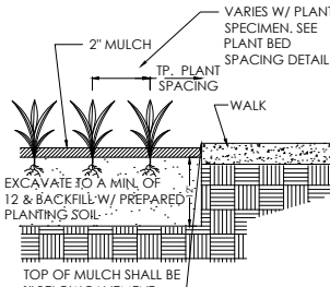
PLANTING DETAIL
