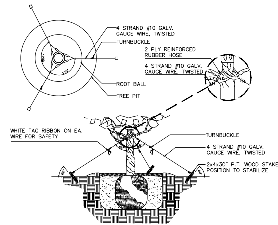
TREE PLANTING AND GUYING DETAIL
