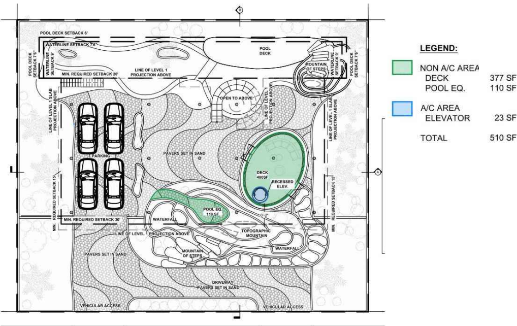
1 A014 UNIT SIZE - UNDERSTORY LEVEL 1/32" = 1'-0"
