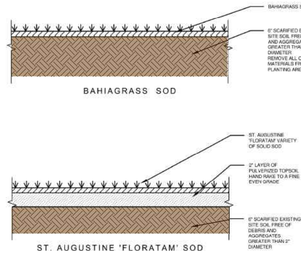
5 SOD PLANTING DETAIL SECTION N.T.S.
