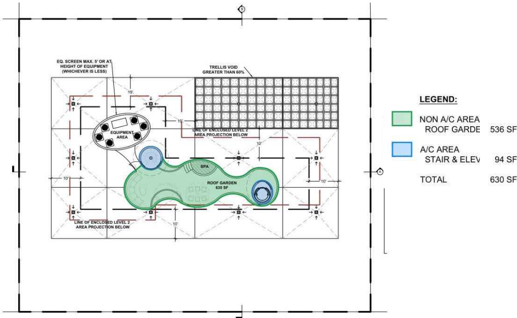
4 A014 UNIT SIZE - ROOF LEVEL 1/32" = 1'-0"
