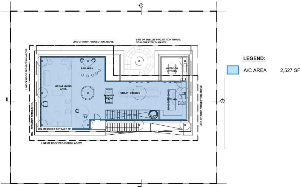
3 A014 UNIT SIZE - LEVEL 2 1/32" = 1'-0"
