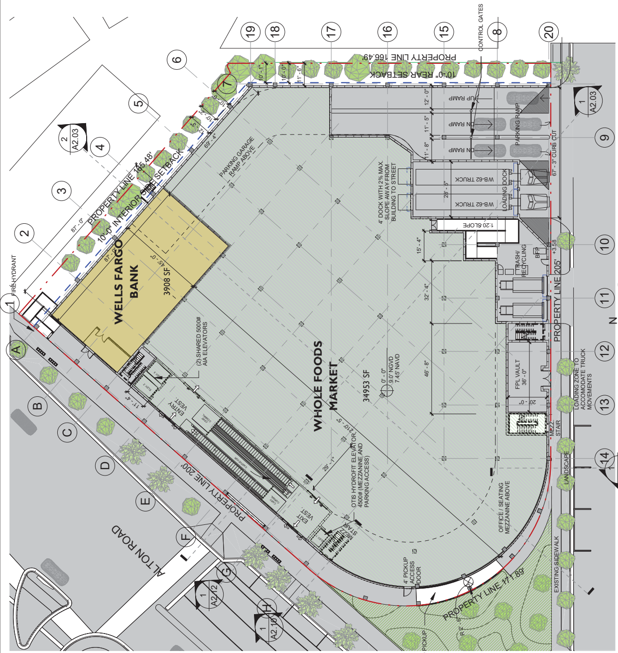
LEVEL 1 FLOOR PLAN 1/32" = 1'-0"
